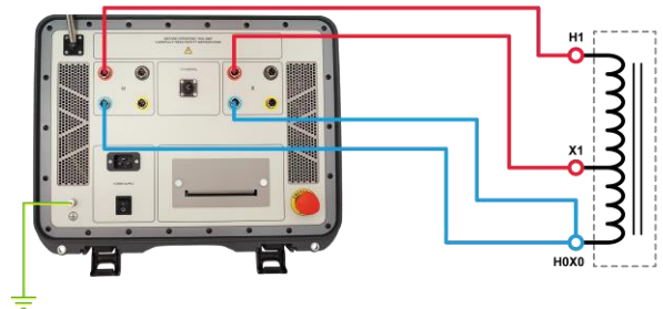
Connecting TRT500 to a single-phase autotransformer
