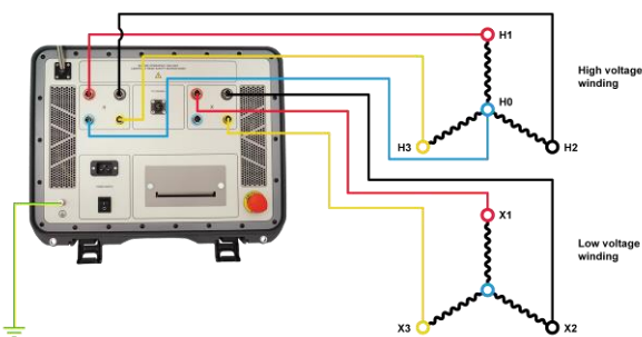
Connecting TRT500 to a three-phase transformer
